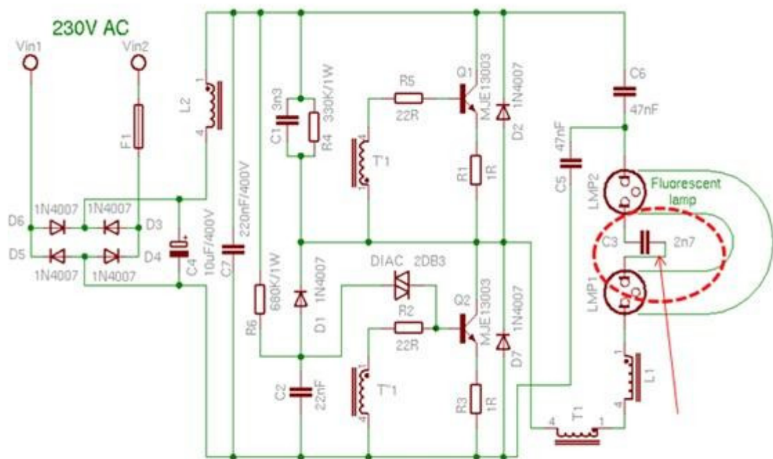
Schematic Diagram Of CFL Bulb
